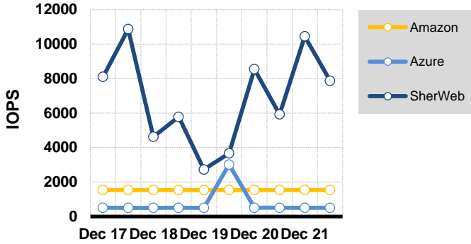
Storage Performance of Sequential Reads (2 vCPU - 32kb)
