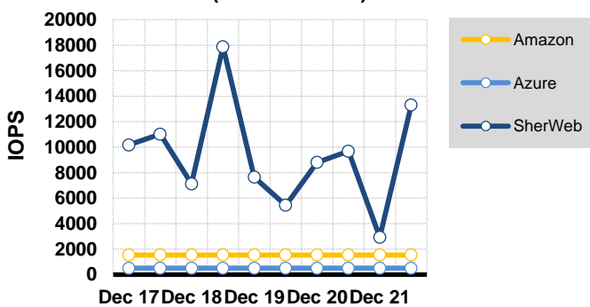
Storage Performance of Sequential Reads (8 vCPU - 32kb)
